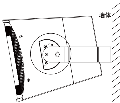
墙壁壁挂
